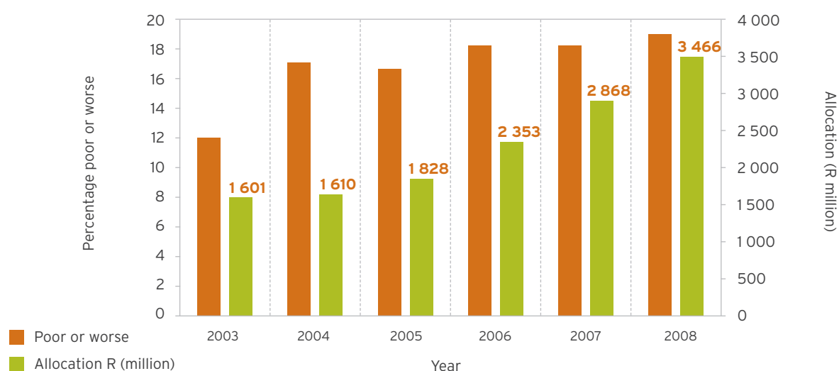
Paved road deterioration and allocations – Northern Cape, North West, Gauteng and Western Cape Provinces
