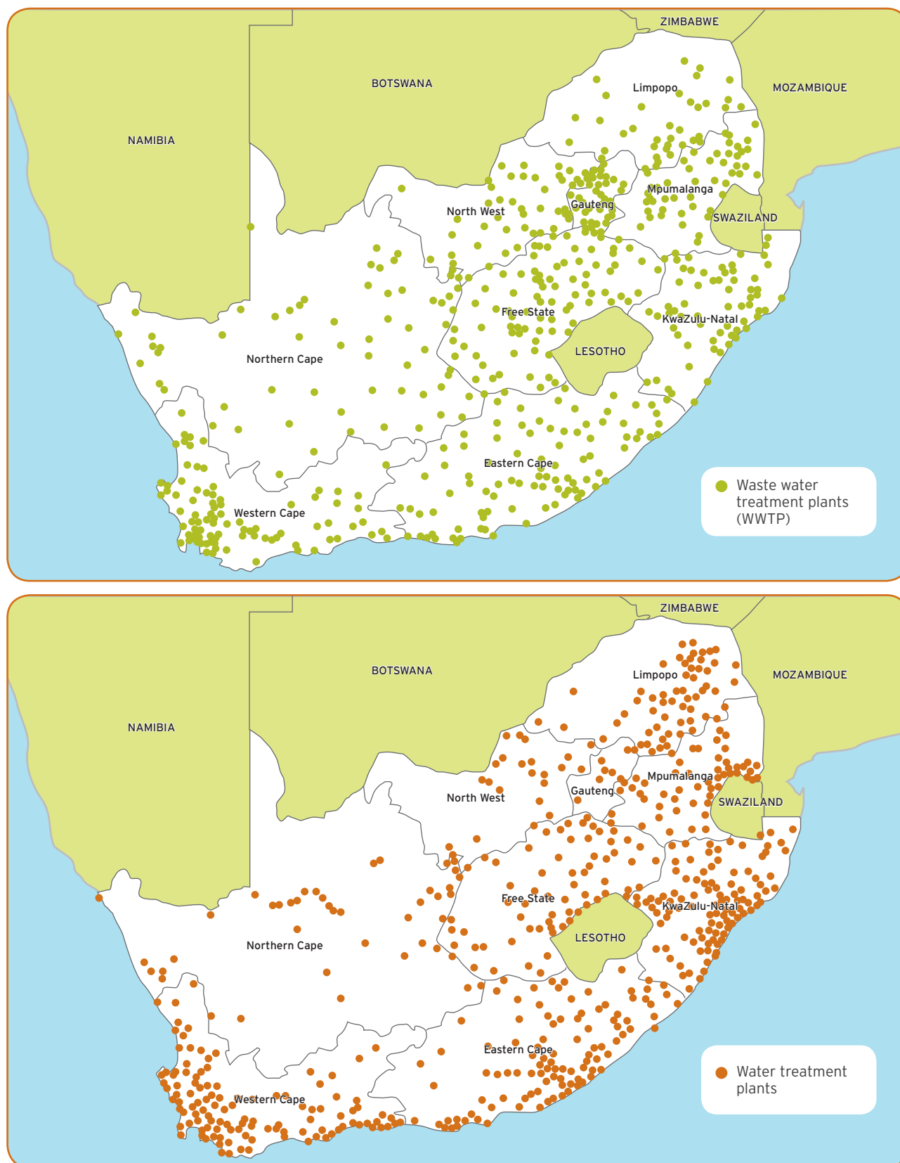
Figure 44: Locations of water (above) and wastewater (below) treatment plants across the country Source: Department of Water Affairs (2011)
