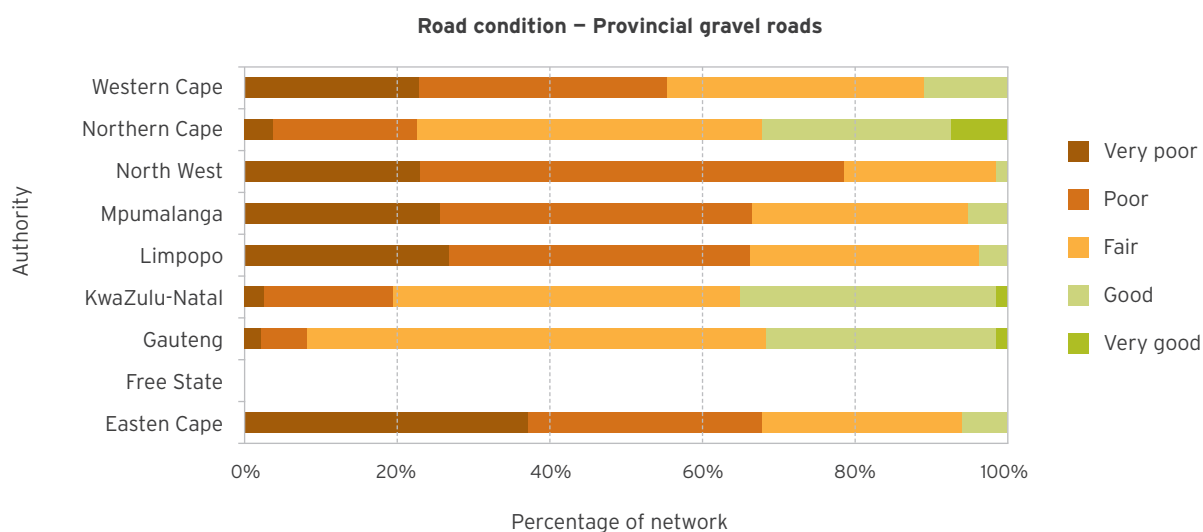
Figure 24: Road condition – Provincial gravel roads
