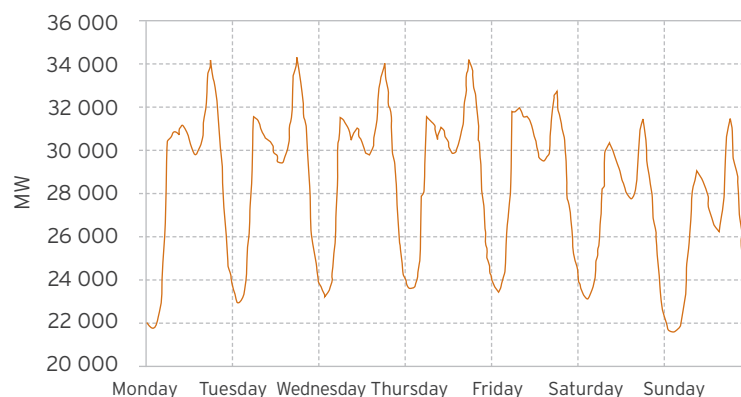
Eskom integrated system hourly peak demand
