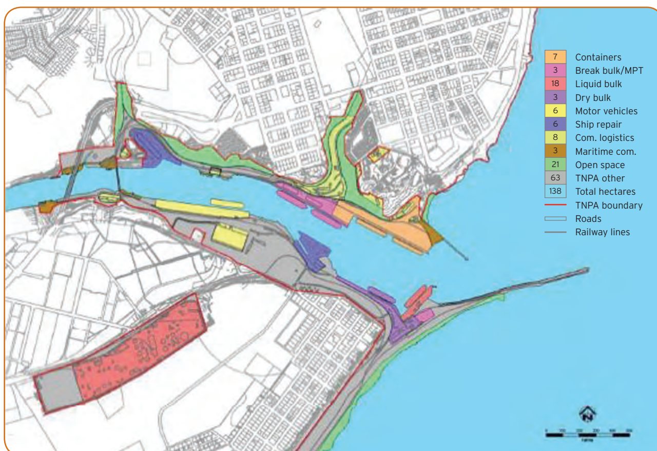
Figure 15: Port of East London, layout of berths and facilities
