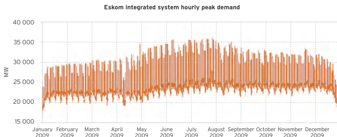
Figure 34: Annual demand for electricity, 2009
